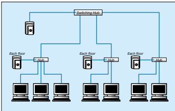
LAN System (Local monitoring system)
