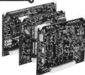
SA-T22U TBC Board for BR-S522U, BR-S622U and BR-S822U/DXU
