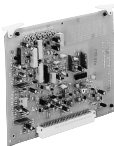
SA-E68U Y/C 688 Output Board for BR-S522U/DXU, BR-S525U/ DXU, BR-S622U/DXU and BR-S822U/DXU
