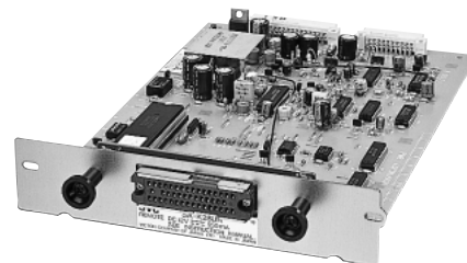
SA-K28UA 45-pin Remote Board for BR-S522U/DXU, BR-S622U/ DXU, BR-S822U/DXU, BR-S800U, BR-S500U and BR-S605UB
