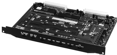
SA-R22U TC Generator/Reader for BR-S522U, BR-S525U, BR-S622U and BR-S822U
